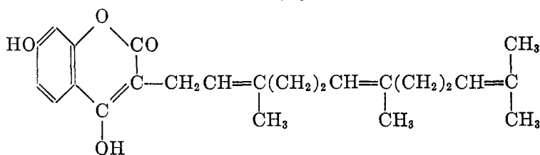
Ammoiresinol
